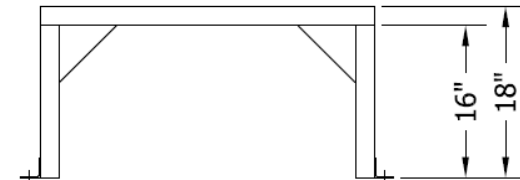
SIDE ELEVATION
