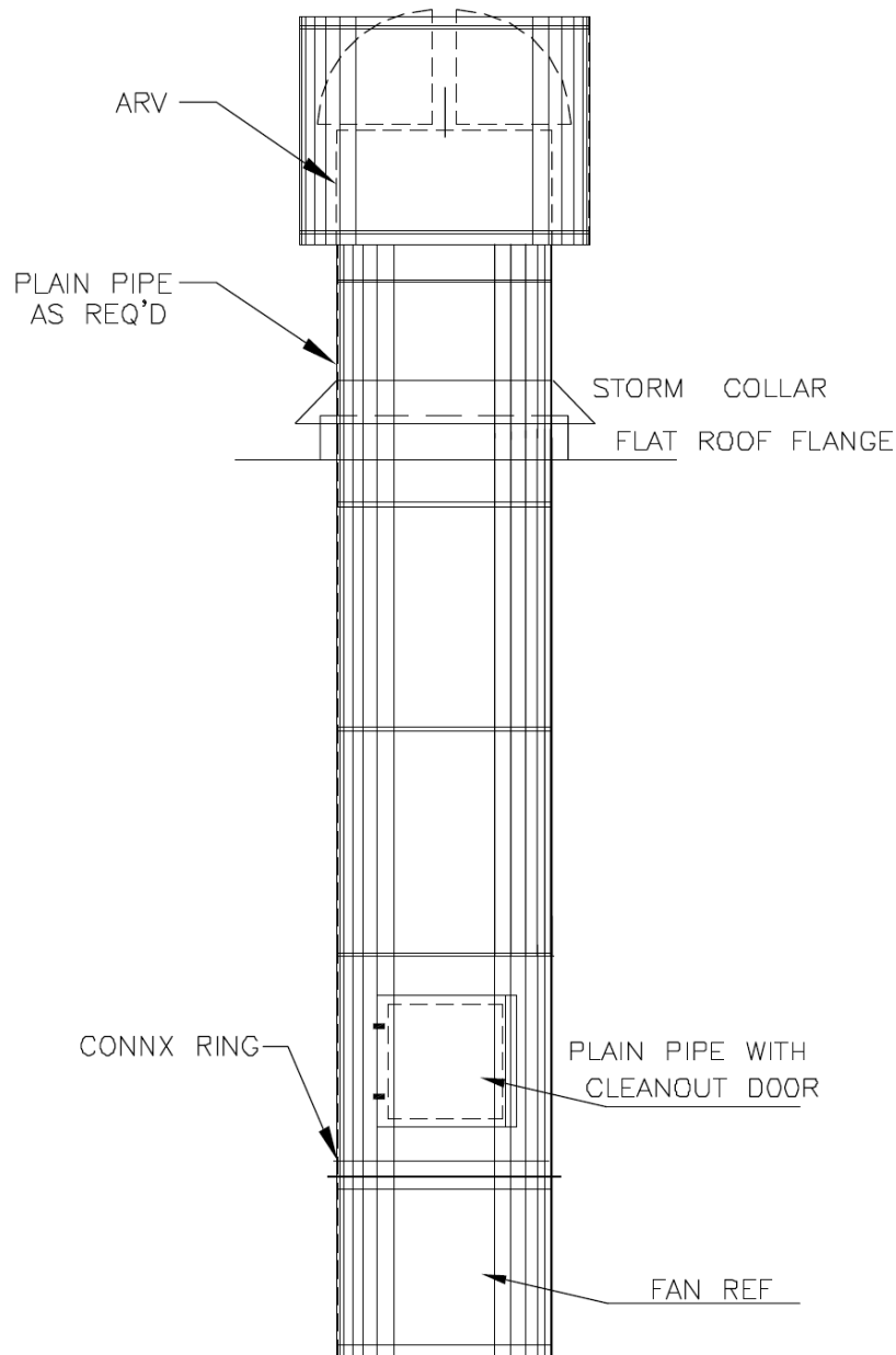
PIPE DETAIL
